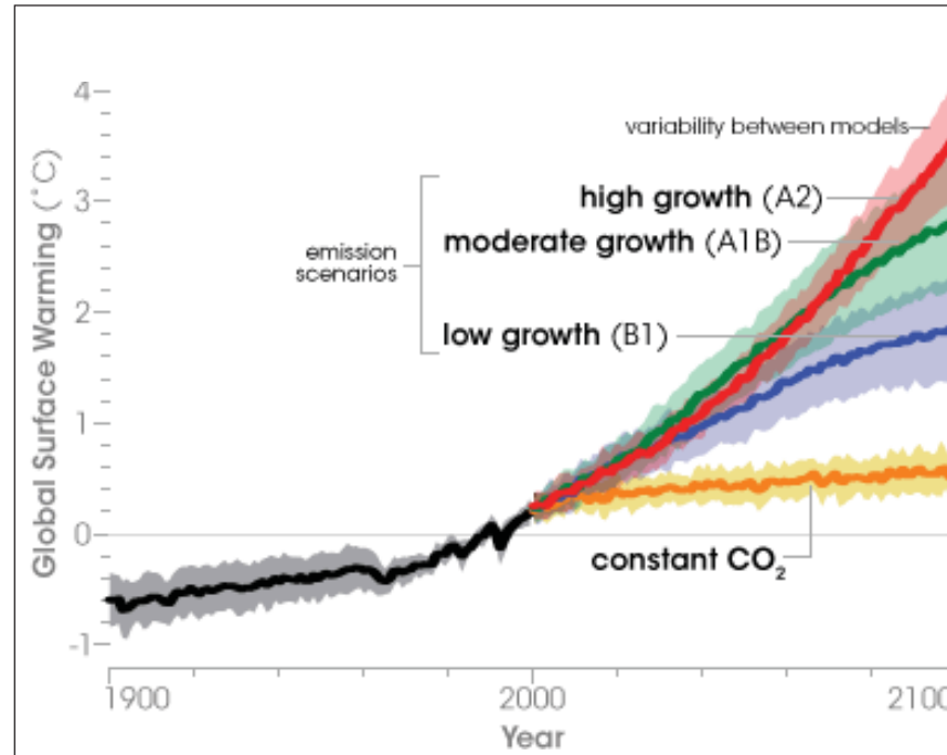
Figure 2: Global Climate Change Projections 9 Temperature projections to the year 2100, based on a range of emission scenarios and global climate models. Scenarios that assume the highest growth in greenhouse gas emissions provide the estimates in the top end of the temperature range. The orange line ("constant CO 2 ") projects global temperatures with greenhouse gas concentrations stabilized at year 2000 levels. A change of 1 degree Celsius is the equivalent of 1.8 degrees Fahrenheit.
