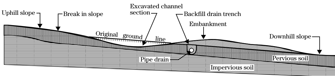
B. - Cross section showing open drain as surface water diversion with pipe drain as subsurface interceptor.
