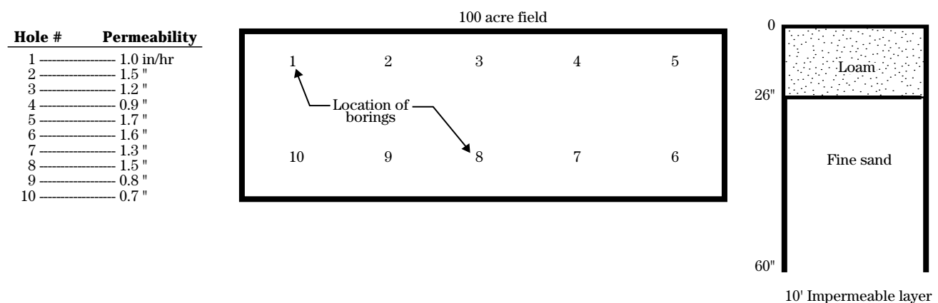
Figure 14-56 Field layout of hydraulic conductivity tests (1 per 10 acres)
