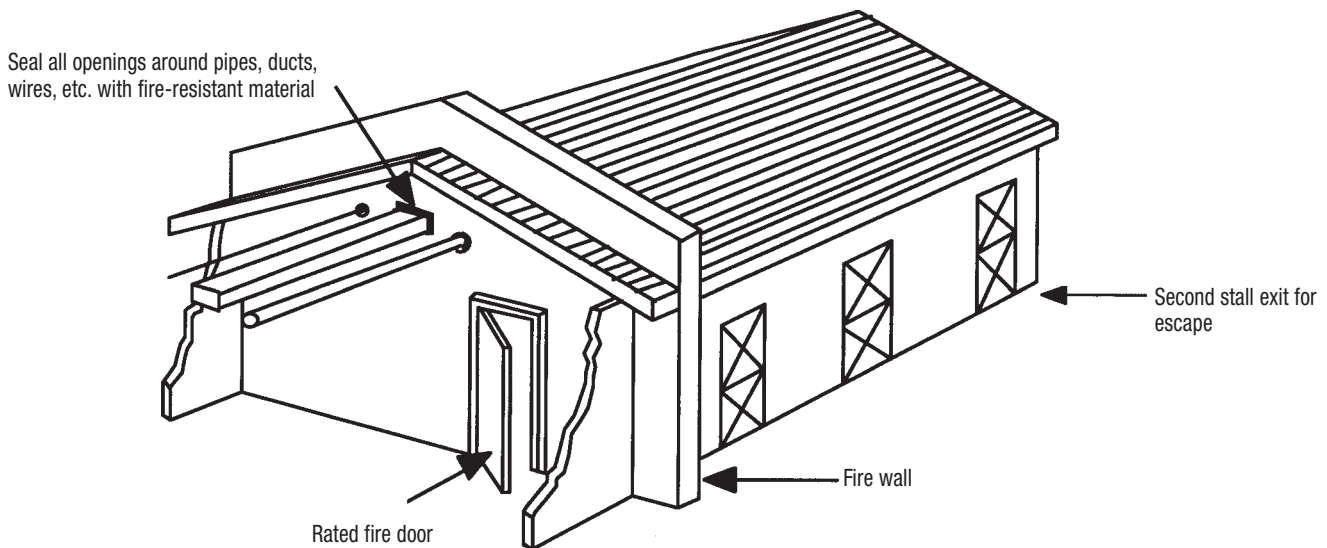
Figure 3. Fire wall to prevent or delay the spread of fire.
