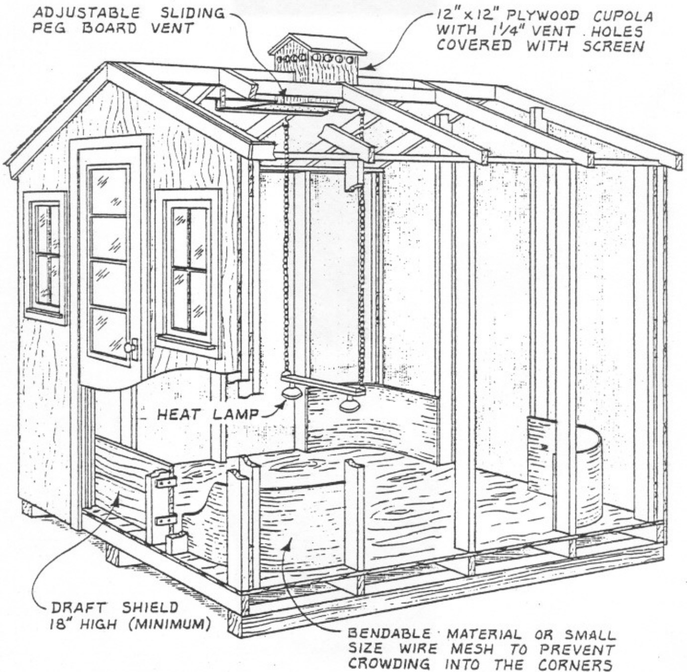
CUTAWAY VIEW
